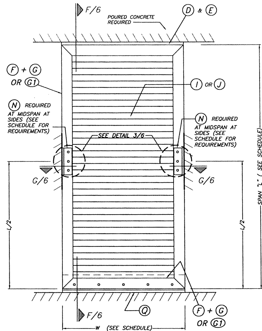
SINGLE UNIT
