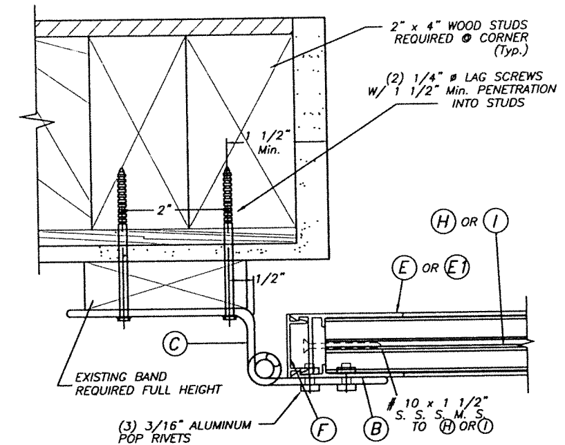
DETAIL 1A (PLAN) SCALE : 1/4" = 1"
