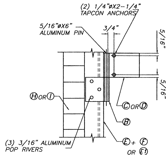
ALTERNATE DETAIL 3
