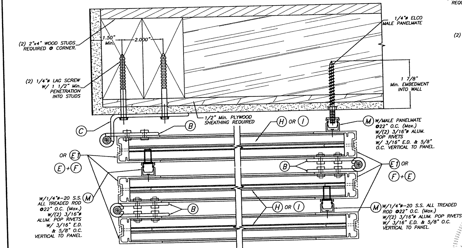
DETAIL 7A: NON HURRICANE POSITION ONLY (PLAN) SCALE : 3/8" = 1"
