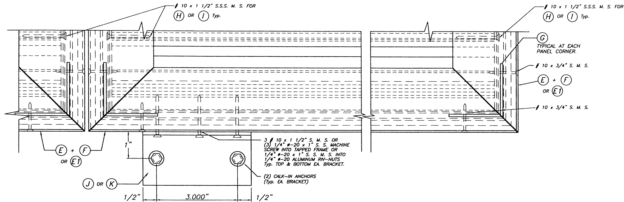
DETAIL 1 SCALE : 1/2" = 1"
