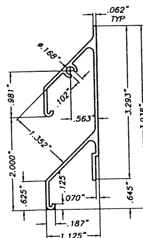
(H) HALF SHUTTER BLADE
