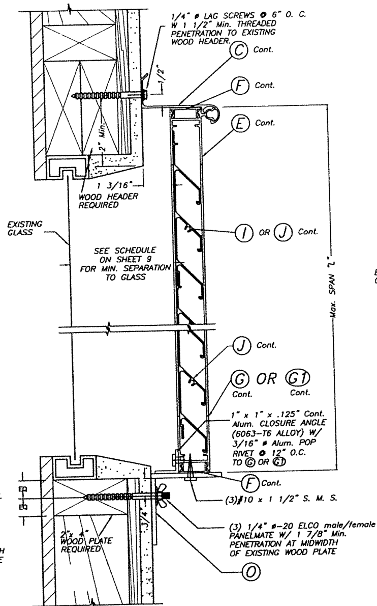
ALTERNATIVE 2 HURRICANE POSITION SCALE: 3/8" = 1"
