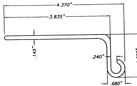
(C) SINGLE HINGE
