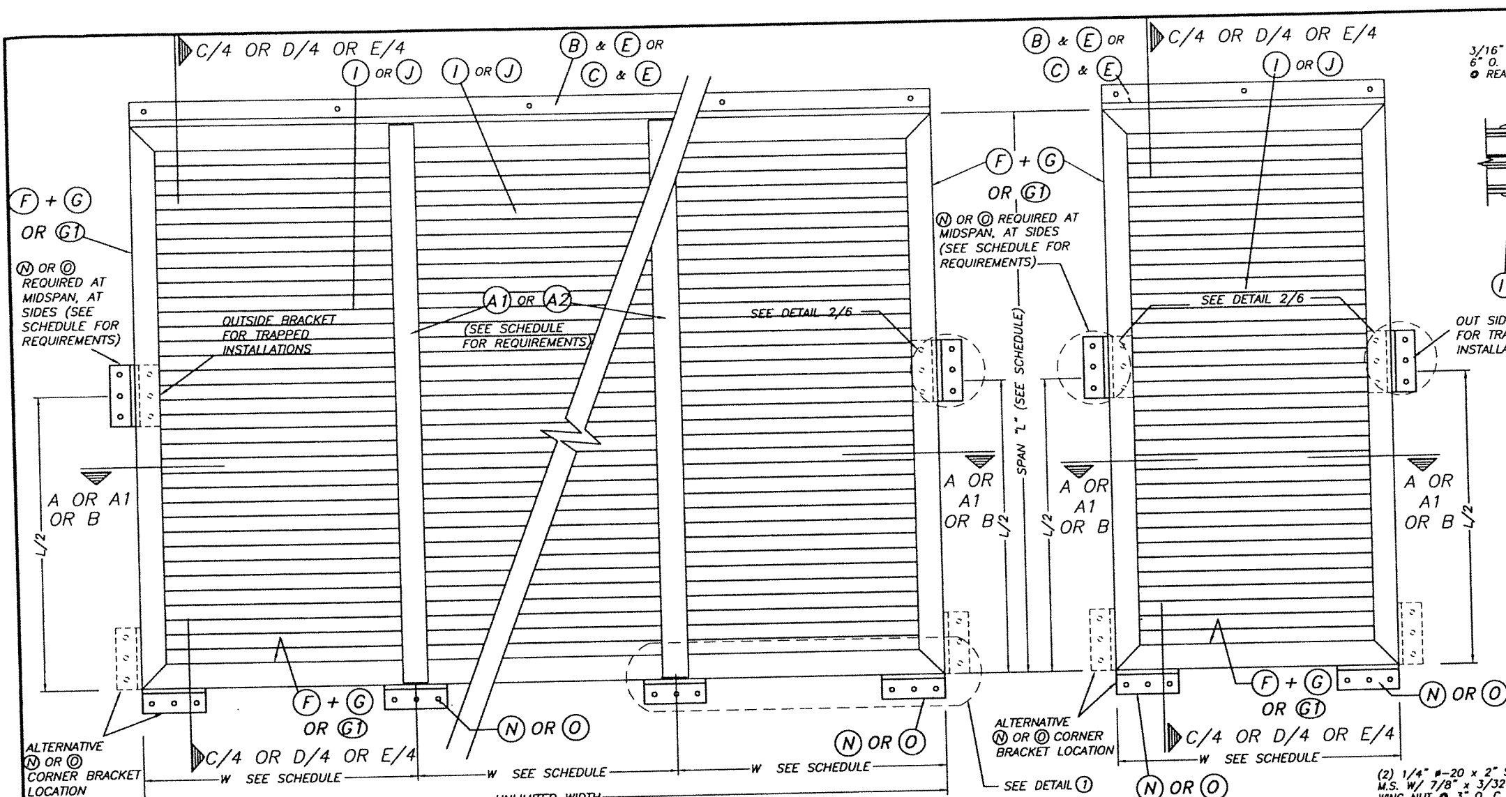
MULTIPLE UNIT
