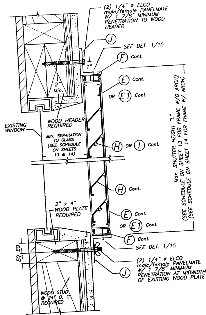
SECTION D' - D' (FLUSH MOUNT) SHUTTER BLADE REVERSELY ORIENTED HURRICANE POSITION SCALE: 1/4" = 1"
