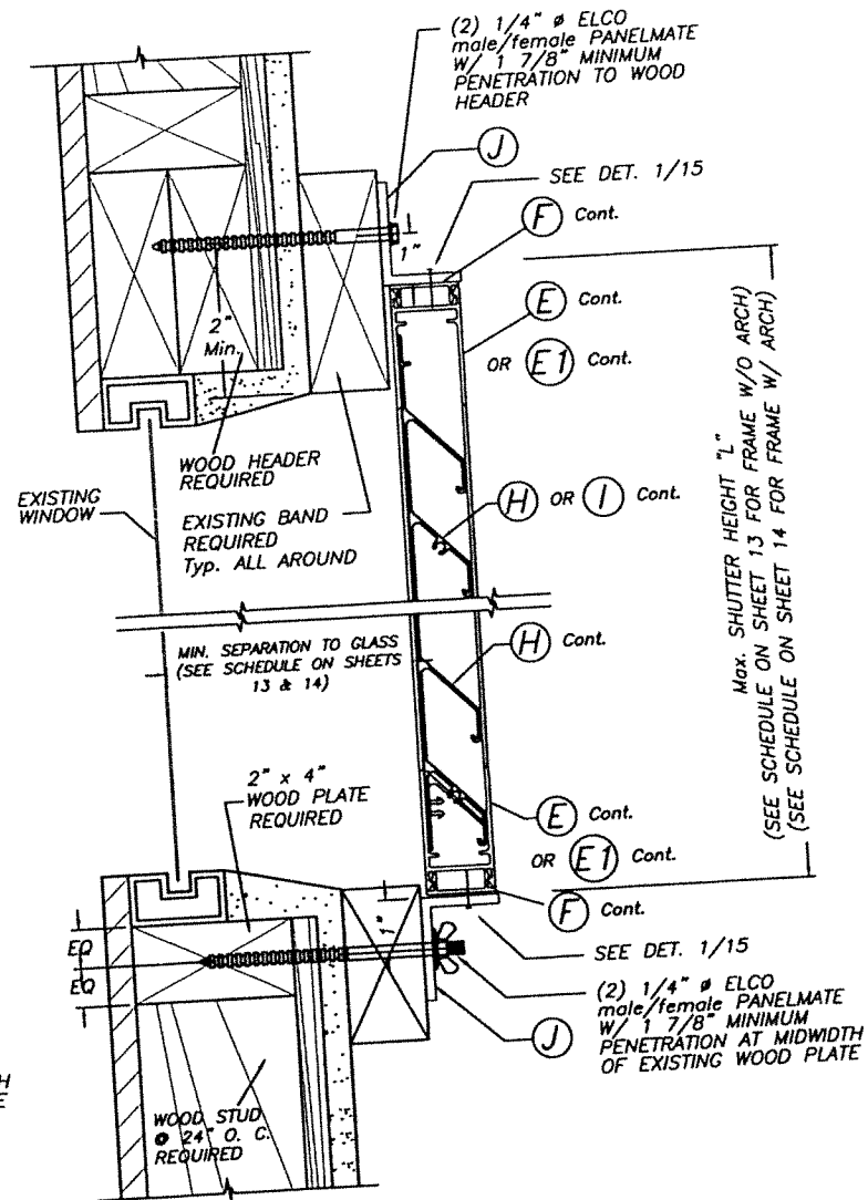
SECTION C' - C' (BUILD-OUT MOUNT) HURRICANE POSITION SCALE: 1/4" = 1"
