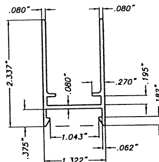
(E) COLONIAL FRAME
