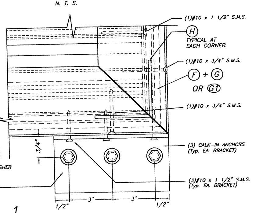
ELEVATIONS
