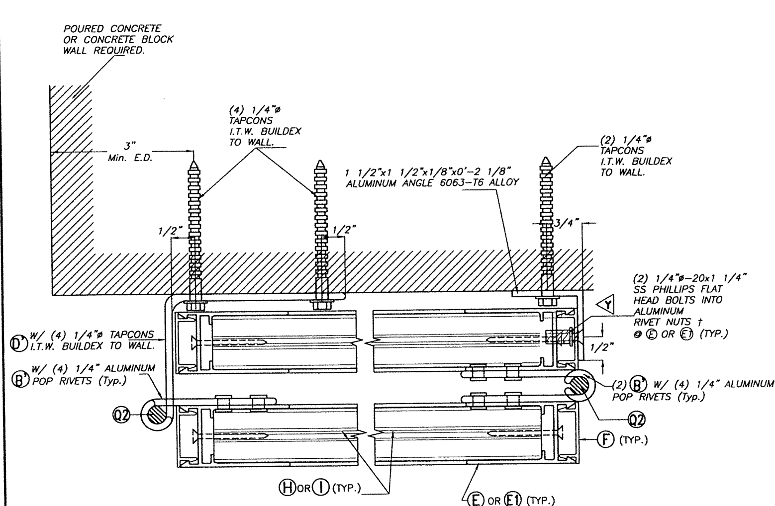
DETAIL X (NON HURRICANE POSITION) SCALE 1/8"=1"
