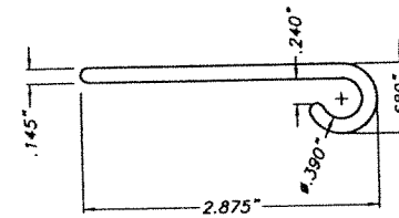
(B') FLAT HINGE
