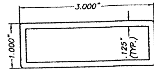
(O1) STORM BAR TYPE 2
