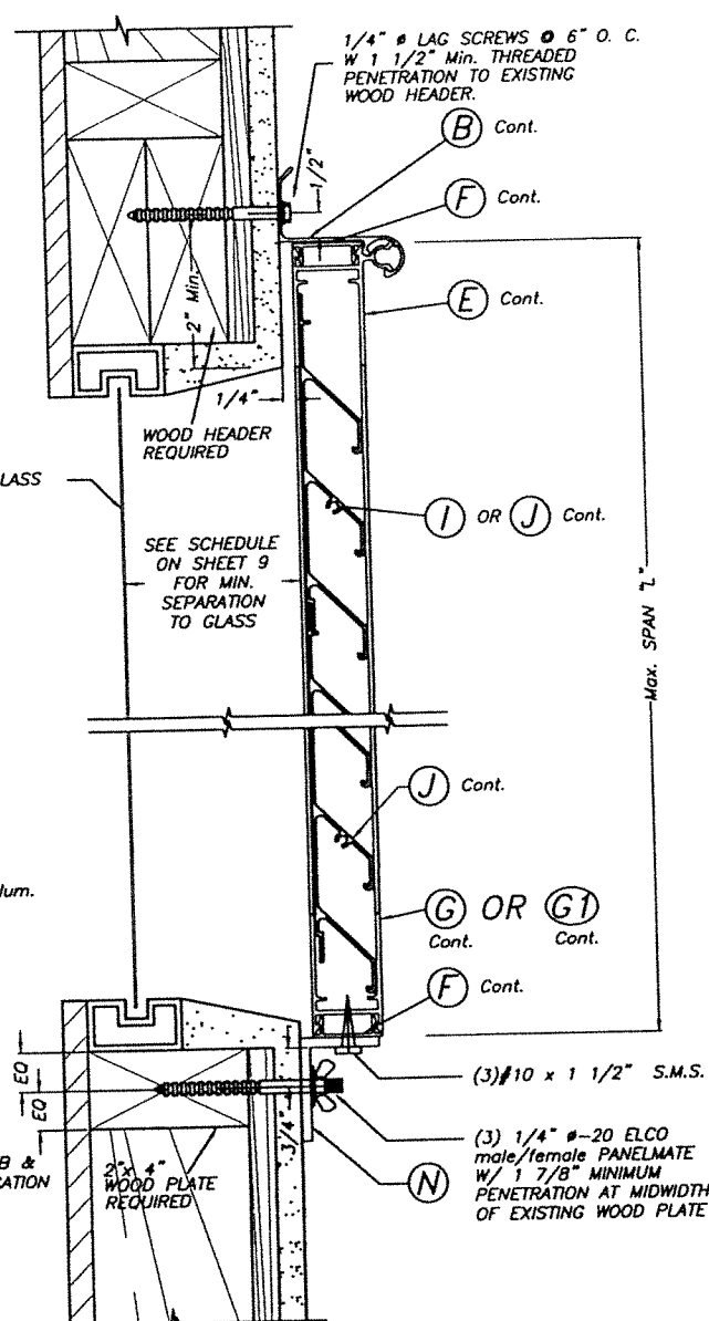
ALTERNATIVE 1 HURRICANE POSITION SCALE: 3/8" = 1"
