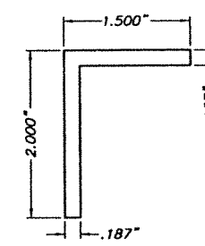
N WALL MOUNT Alum. BRACKET 7" LONG SCALE: 1/2" = 1"
