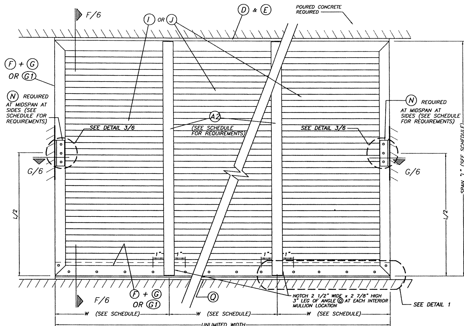
MULTIPLE UNIT
