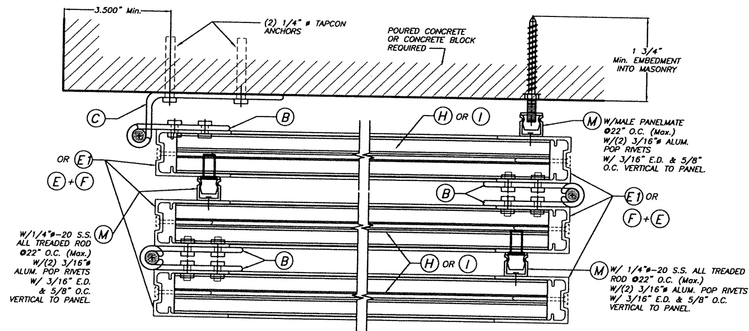
DETAIL 7: NON HURRICANE POSITION ONLY FOR INSTALLATION AT QUADRUPLE PANEL ONLY (PLAN) SCALE : 3/8" = 1"
