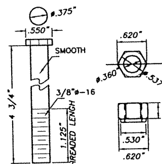
(Q2) ALUMINUM PIN FOR HINGE 6061-T6 Alum. ALLOY
