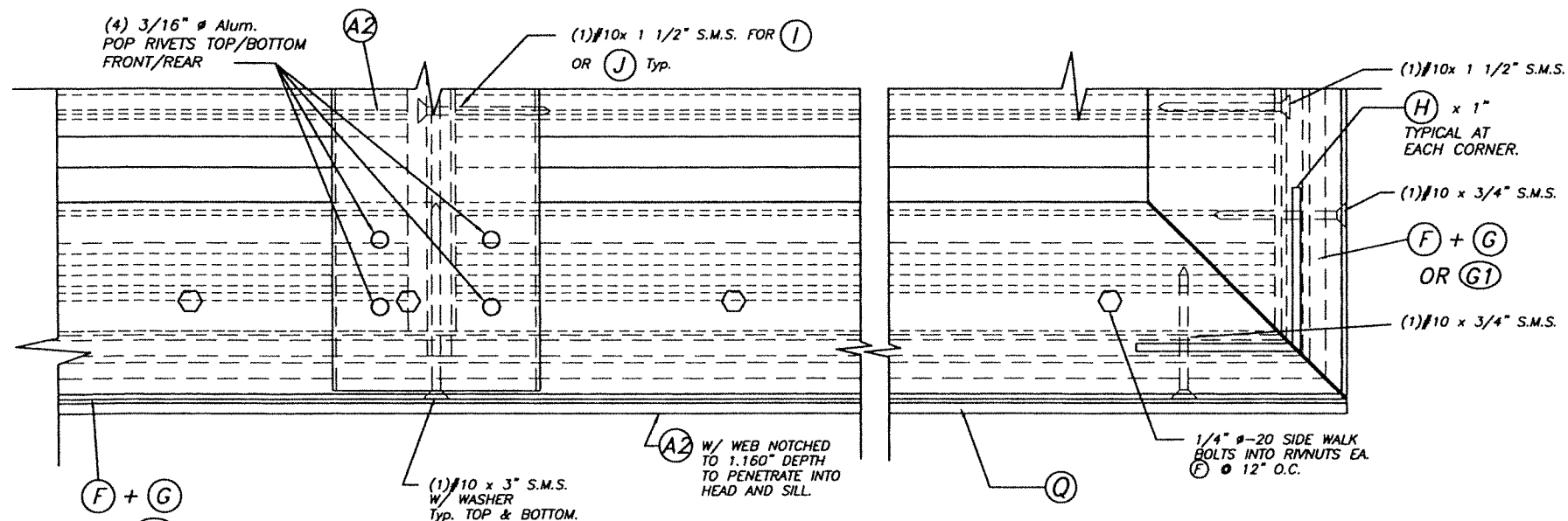
DETAIL 1
