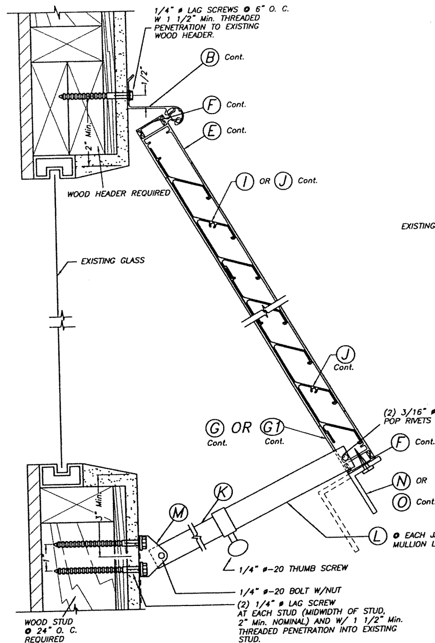
NON HURRICANE POSITION DETAIL: (74 m.p.h. OR LESS WIND SPEED) SCALE: 3/8" = 1"
