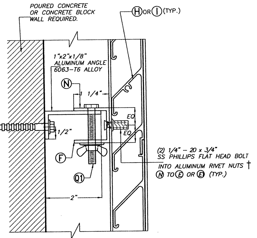
ELEVATION Y-Y
