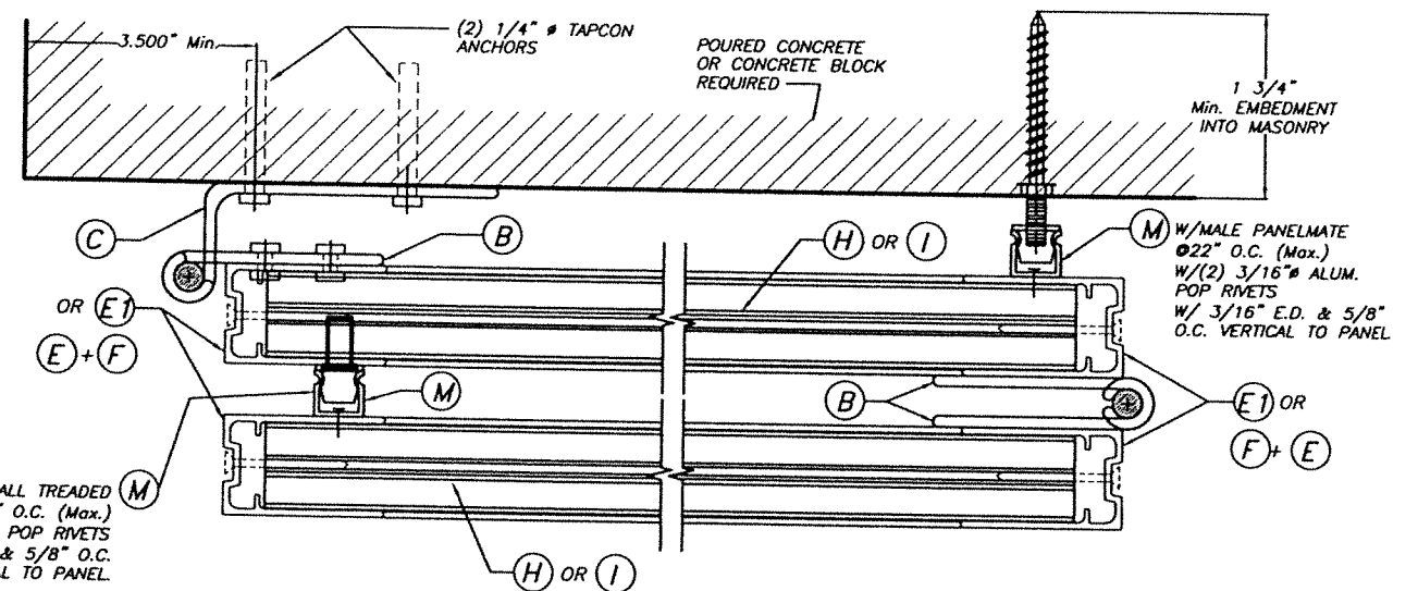
DETAIL 8: NON HURRICANE POSITION ONLY (PLAN) SCALE : 3/8" = 1"
