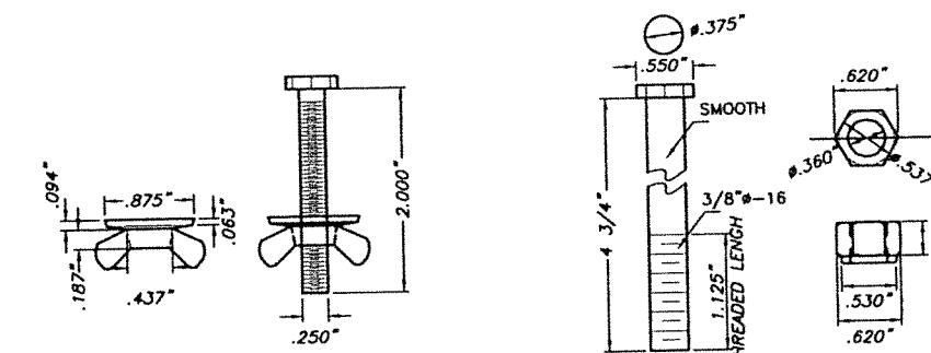
(Q2) ALUMINUM PIN FOR HINGE 6061-T6 Alum. ALLOY
